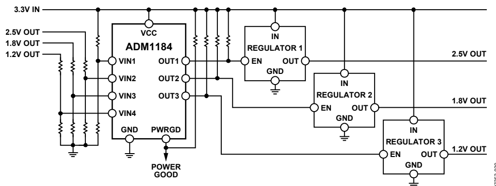
Figure 20. Voltage-Monitoring and Sequencing Application Diagram
