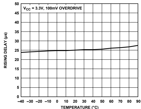
Figure 7. VIN1/VIN2/VIN3 to OUT1/OUT2/OUT3 Rising Delay vs. Temperature
