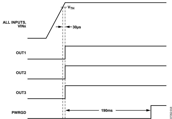
Figure 18. Power-Up Waveforms
