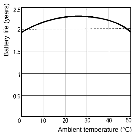
Battery Service Life vs. Temperature
