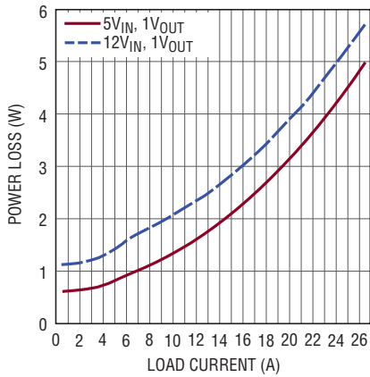
Figure 12. 1.0V Power Loss Curve
