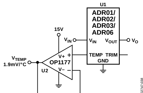
Figure 37. Temperature Monitoring
