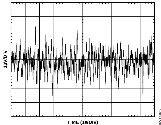
Figure 24. ADR02 Typical Noise Voltage 0.1 Hz to 10.0 Hz
