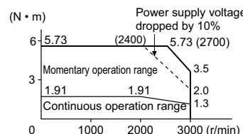
R88M-K40020F/C (400 W)
