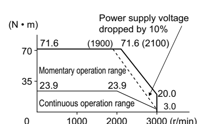
R88M-K5K020(H/T)-□ (5 kW)
