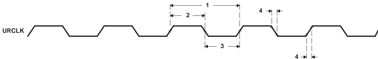
Figure 58. URCLK Timing
