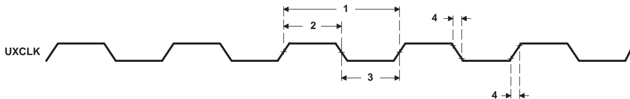
Figure 57. UXCLK Timing
