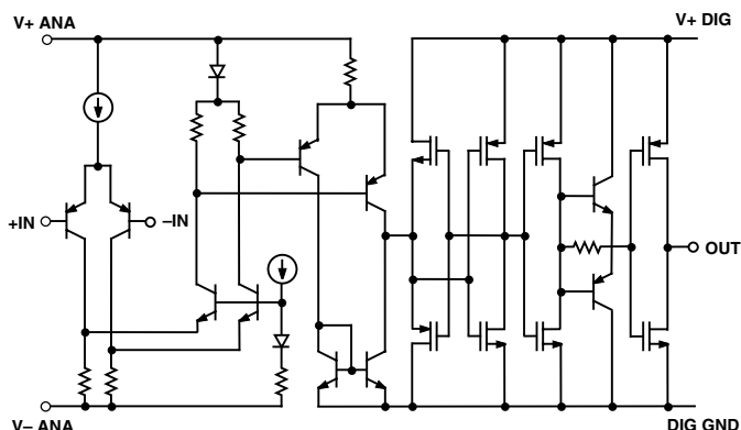
Figure 1. Simplified Schematic
