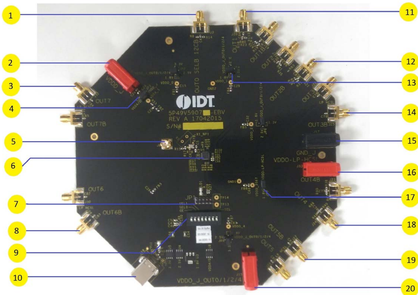
Figure 1. Board Overview
