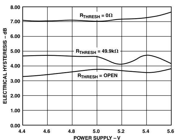
TPC 5. Signal Detect Hysteresis vs. Power Supply
