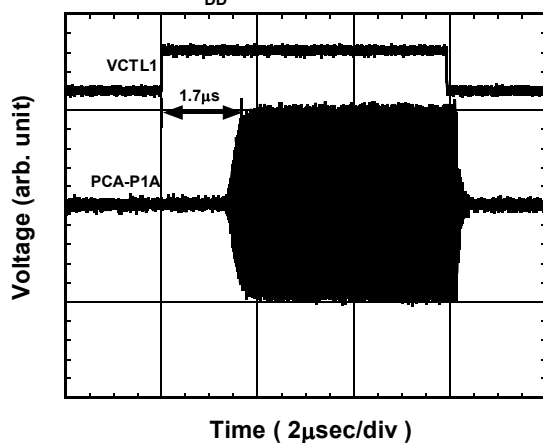
Switching Time
