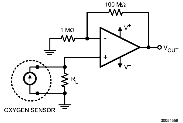
FIGURE 4. Precision Oxygen Sensor
