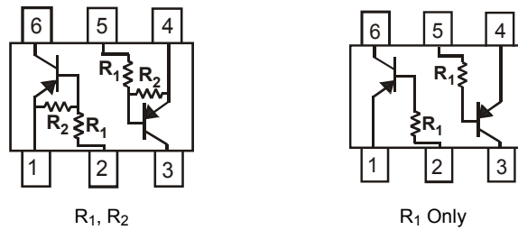
SCHEMATIC DIAGRAM
