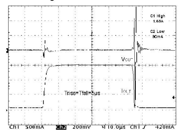
Figure 27. Load transient
