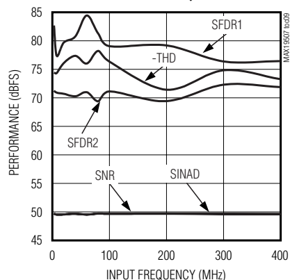
PERFORMANCE vs. INPUT FREQUENCY
