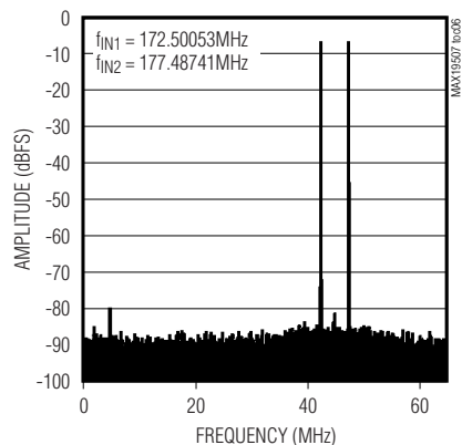
175MHz TWO-TONE IMD PLOT
