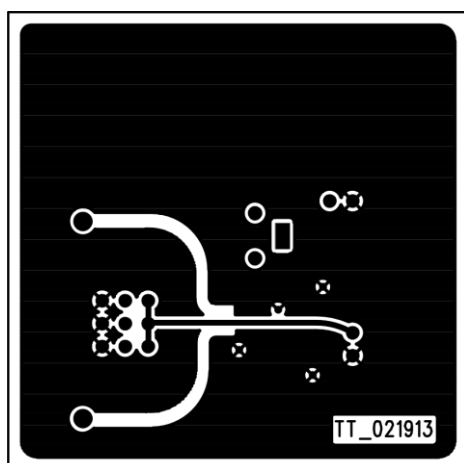
Figure 5. Bottom Layer (GND) #2
