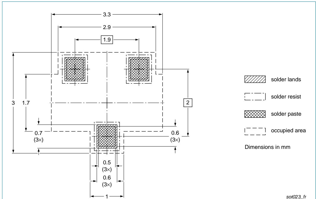
Fig 18. Reflow soldering footprint PDTA114ET (SOT23)
