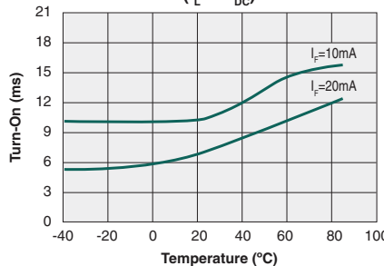
Typical Turn-On vs. Temperature ( I_L=1\text{A}_{DC} )
