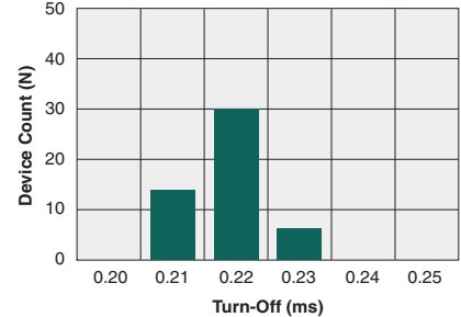
Typical Turn-Off Time (N=50, I_F=20\text{mA} , I_L=1\text{A}_{DC} , T_A=25^\circ\text{C} )
