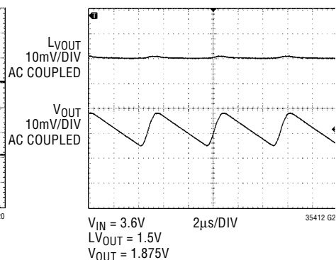
Linear Regulator to VLDO Transition, Load = 30mA
