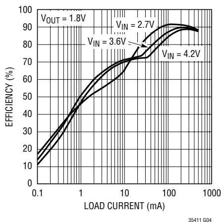
Efficiency vs Load Current for Buck (Pulse Skip)
