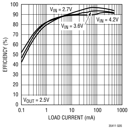
Efficiency vs Load Current for Buck (Burst)
