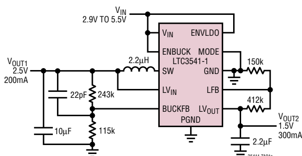
LTC3541-1 Typical Application
