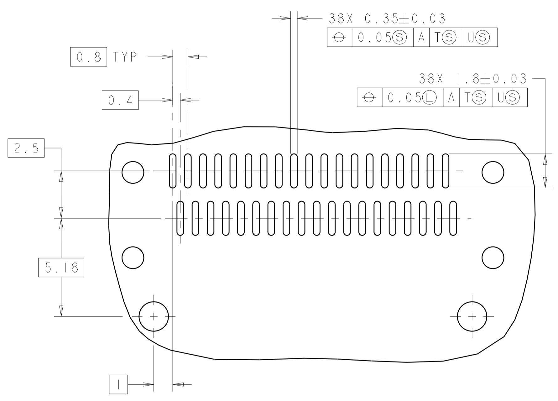
DETAIL K SCALE 8:1
