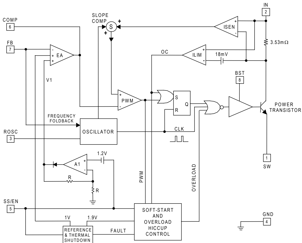
Figure 2 — SC4525EM Block Diagram
