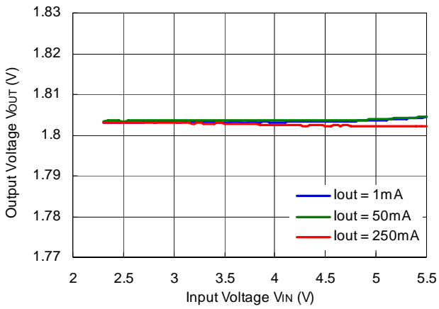
RP507K001B V_{out}=1.8V
