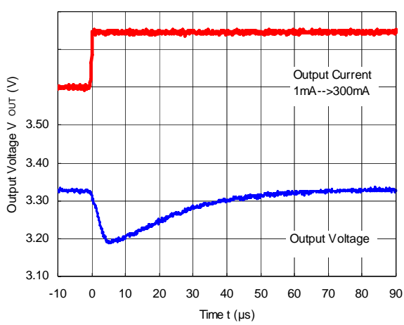
RP550K001A ( V_{IN}=5.0V , V_{OUT}=3.3V ) MODE="H" Forced PWM Control
