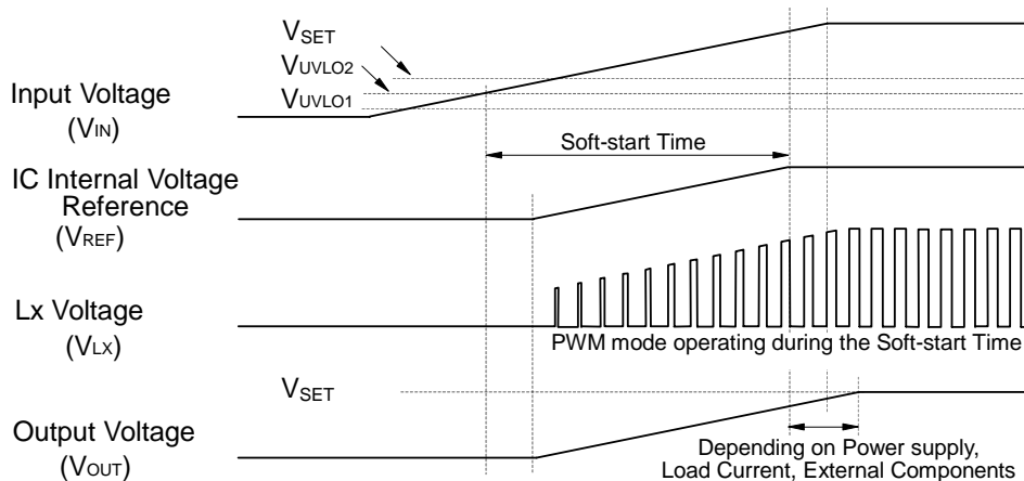
Figure 10. Timing Chart
