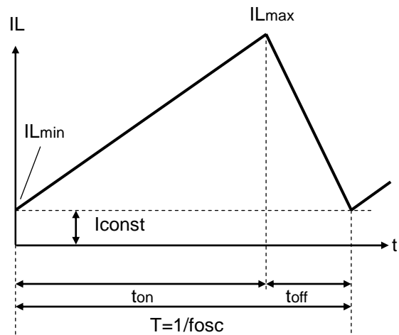
Figure 6. Continuous Mode
