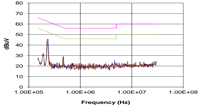
CRE1S0505MEC
