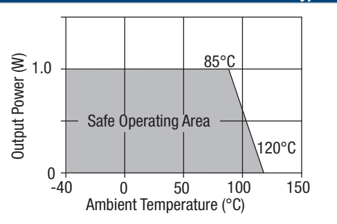
TEMPERATURE DERATING GRAPH - All other types 1
