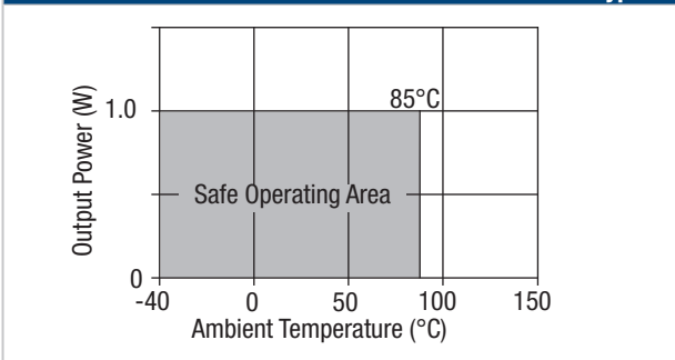
TEMPERATURE DERATING GRAPH - Surface Mount & 3C types
