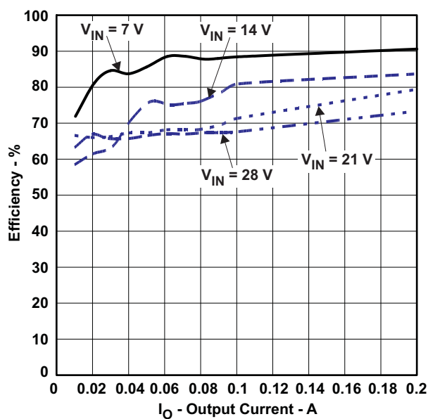
Figure 16. TPS54331 Low Current Efficiency
