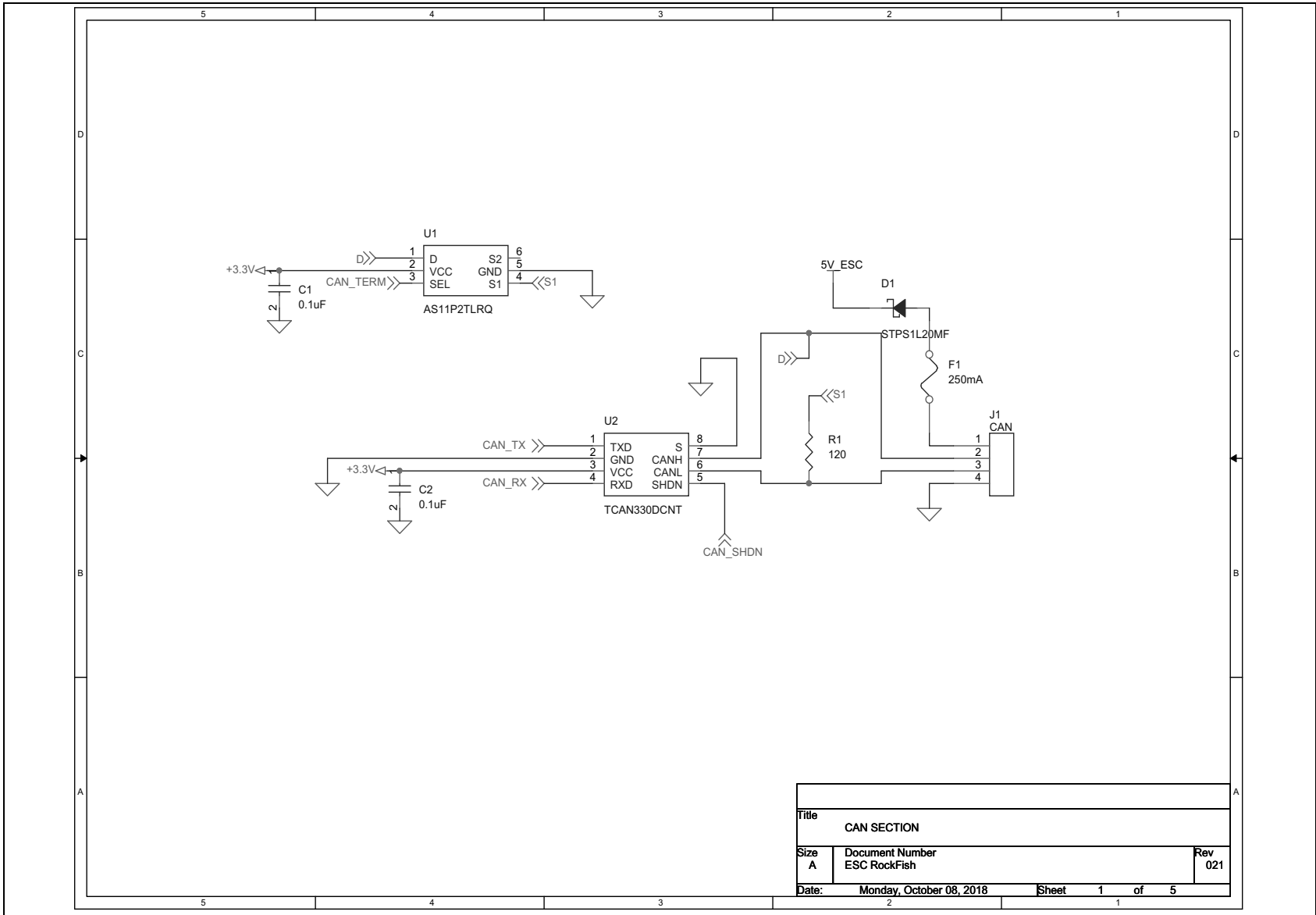
Figure 17. CAN section
