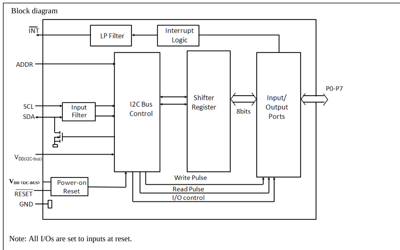
Fig 5: Block diagram
