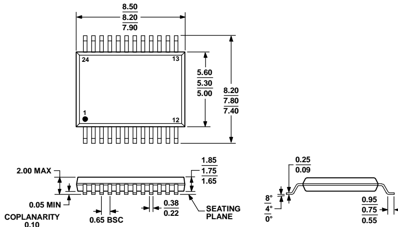
COMPLIANT TO JEDEC STANDARDS MO-150-AG Figure 35. 24-Lead Shrink Small Outline Package [SSOP] (RS-24) Dimensions shown in millimeters
