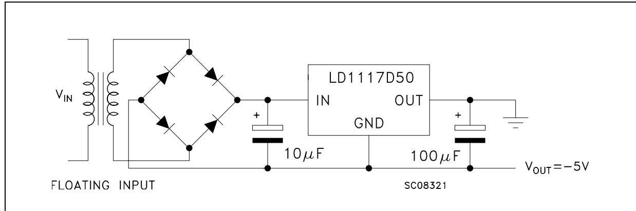
Figure 4. Negative supply
