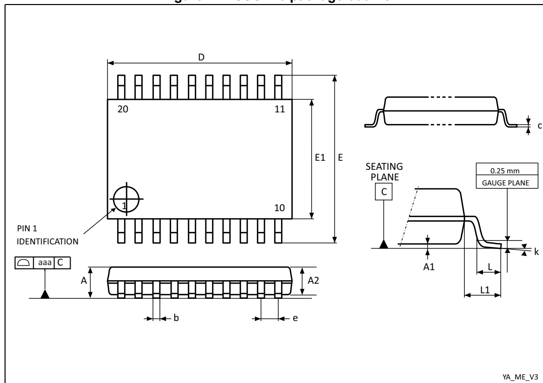
Figure 42.TSSOP20 package outline
