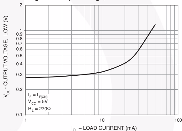
Figure 4. Output Voltage, Low vs. Load Current
