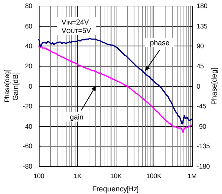
Figure 38. Loop Response ( V_{IN}=24V , V_{OUT}=5V , I_{OUT}=2.5A , C_{OUT}=\text{Ceramic}22\mu F \times 2 )
