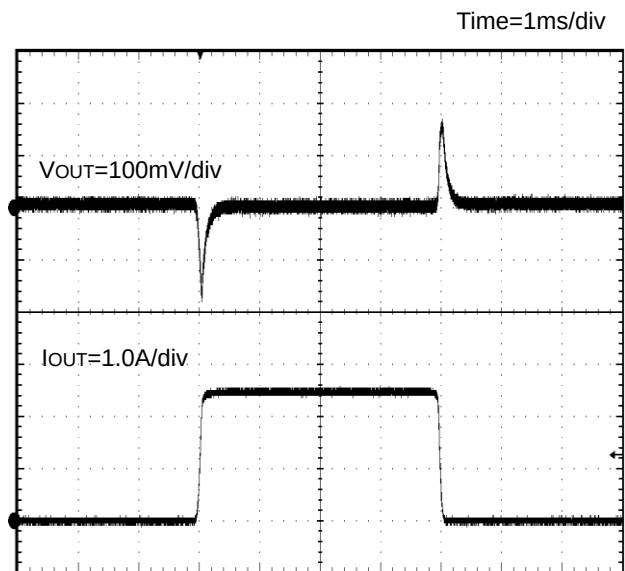
Figure 40. Load Transient Response I_{OUT}=0A - 2.5A ( V_{IN}=24V , V_{OUT}=5.0V , C_{OUT}=\text{Ceramic}22\mu F \times 2 )
