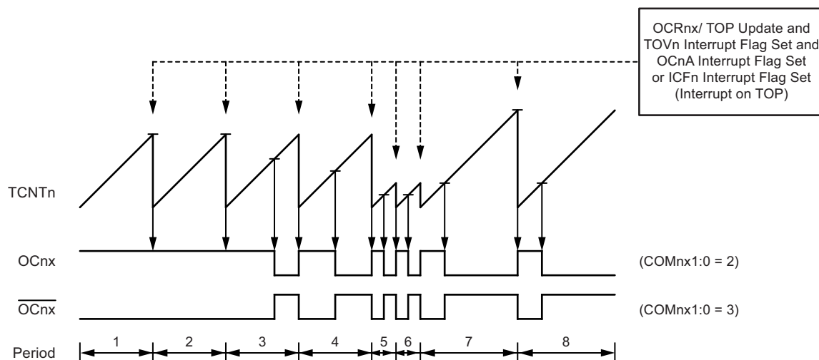
Figure 4-43. Fast PWM Mode, Timing Diagram
