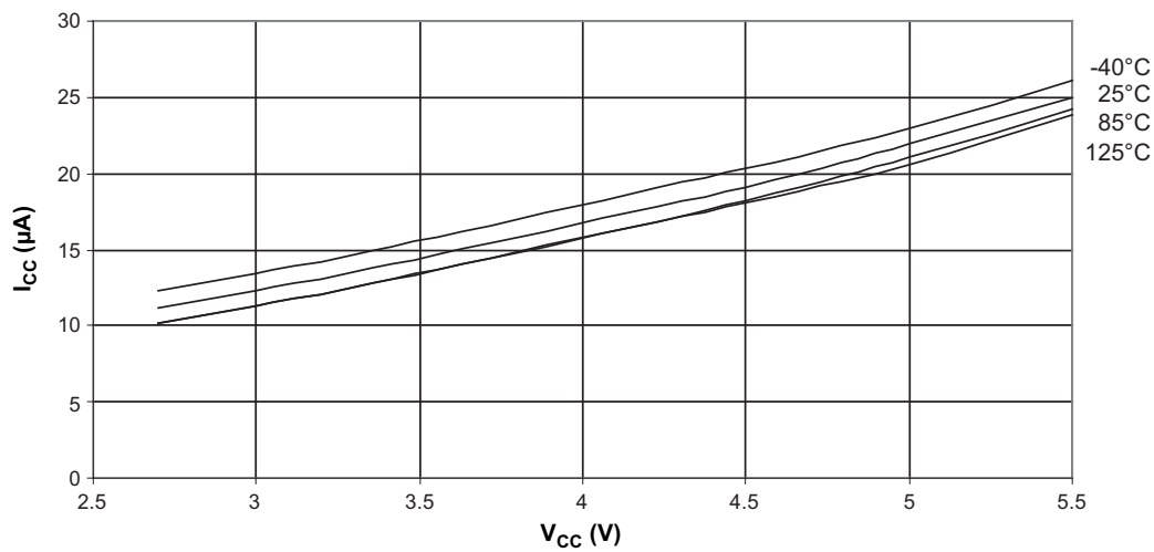
Figure 8-36. Watchdog Timer Current versus V_{CC}
