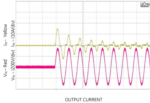
Figure 2. Inrush current V_{IN} = 230V_{AC} , 0^\circ phase angle
