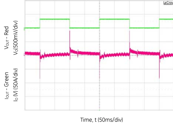
Figure 8. Transient response 54V DC load step 10 – 60%, Slew rate: 1A/ \mu s, V_{IN} = 230V AC .
