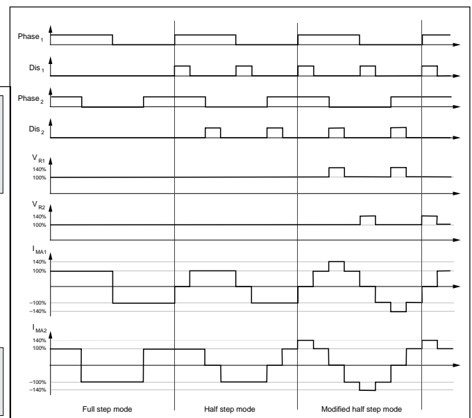
Figure 9. Stepping modes
