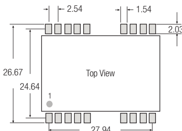
Bottom View Tol.: \pm 0.35 mm Pin area 0.1 x 0.50 23.40 11 x 2.54 0.50 1 2 3 4 5 9 10 11 12 16 15 14 13 24 23 22 21 20
