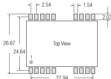
Bottom View Pin area 0.1 x 0.50 Tol.: \pm 0.35 mm 0.50 23.40 11 x 2.54 1 2 3 4 5 9 10 11 12 16 15 14 13 24 23 22 21 20
