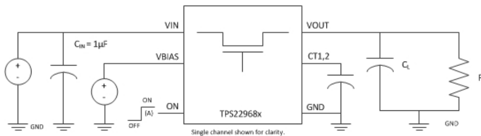
TEST CIRCUIT
