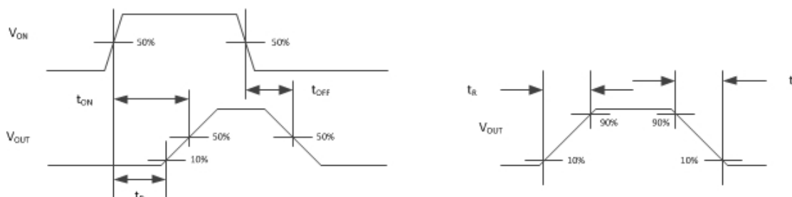
TIMING WAVEFORMS
