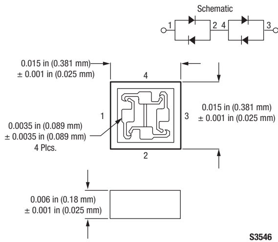
Figure 4. 551-056 Package Dimensions
