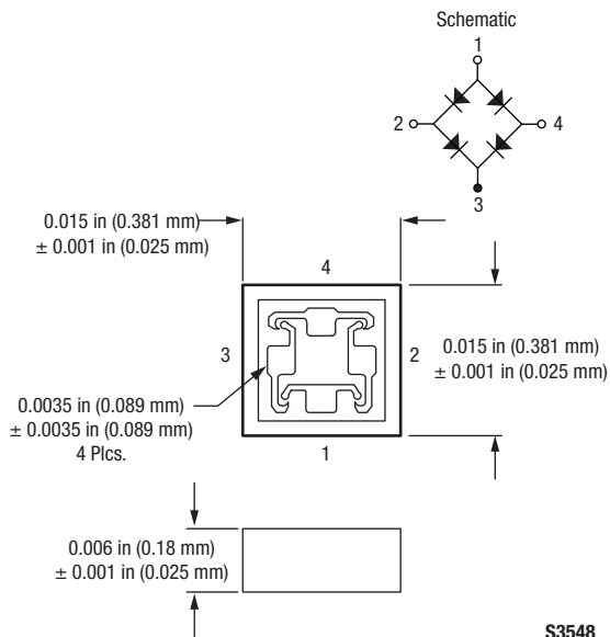
Figure 7. 551-004 Package Dimensions
