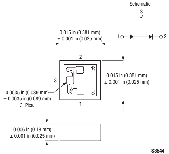
Figure 3. 551-012 Package Dimensions
