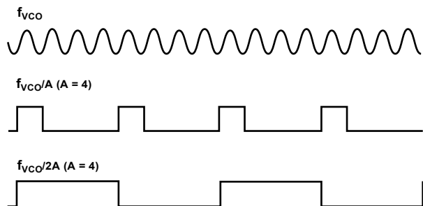
Figure 21. DIVOUT Waveforms
