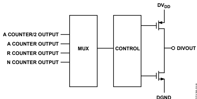
Figure 20. DIVOUT Circuit
