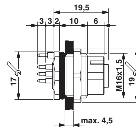
Dimensioned drawing
