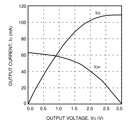
Figure 103. Fast ( T_J = 125\text{ }^{\circ}\text{C} , V_{DD} = 3.0\text{ V} )
