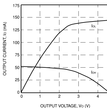
Figure 97. Fast ( T_J = 125^\circ\text{C} , V_{DD} = 4.5\text{ V} )
