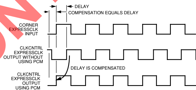
Figure 47. ExpressCLK Delay Minimization Using the PCM
