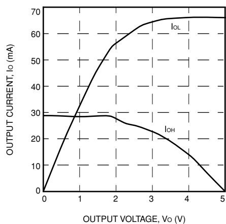
Figure 92. Sinklim ( T_J = 25^\circ\text{C} , V_{DD} = 5.0\text{ V} )
