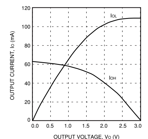
Figure 103. Fast ( T_J = 125\text{ }^{\circ}\text{C} , V_{DD} = 3.0\text{ V} )
