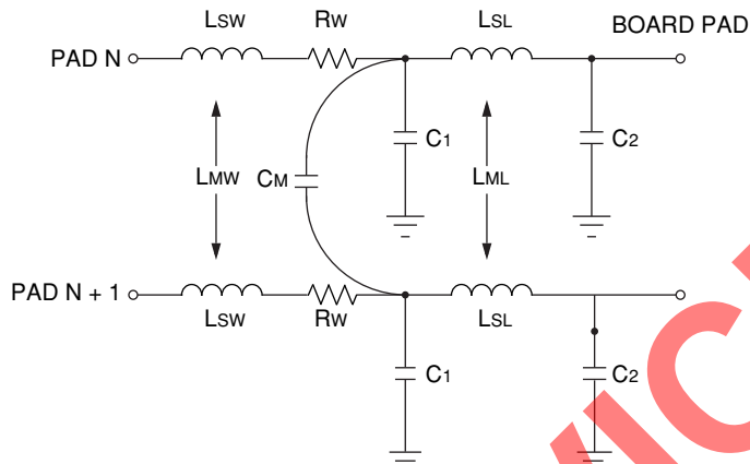
Figure 104. Package Parasitics
