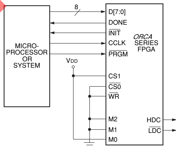
Figure 62. Slave Parallel Configuration Schematic
