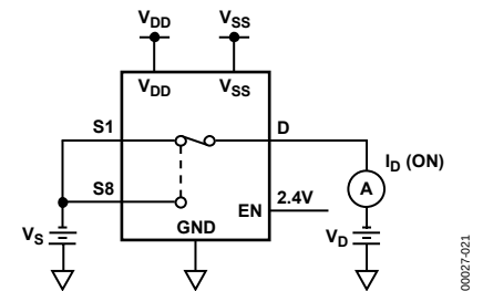
Figure 21. I_D (ON)
