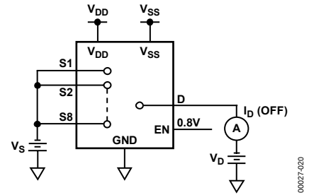
Figure 20. I_D (OFF)
