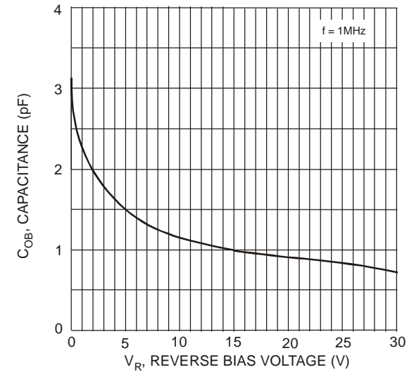
Fig. 4 Output Capacitance
