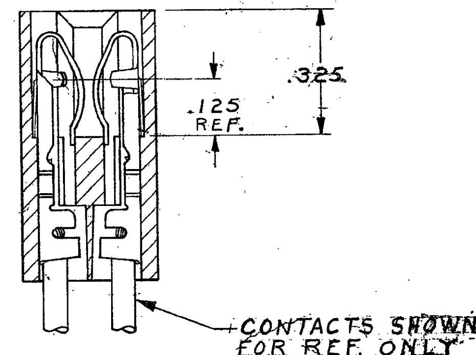
SECT. A-A
